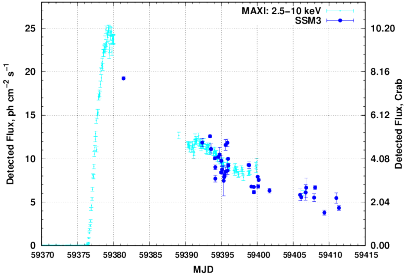
4U 1543-47 with AstroSat/SSM
